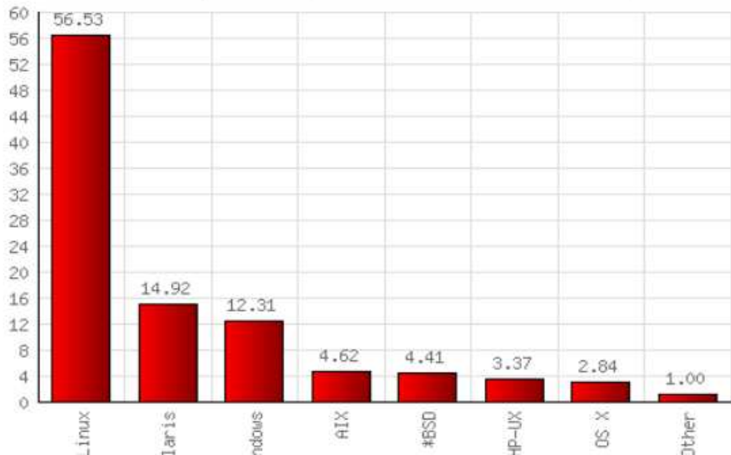
Cfengine.com registered hosts OS distribution
